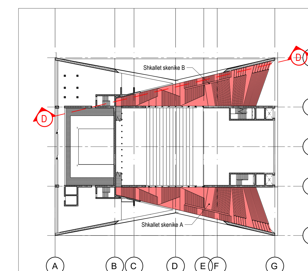
PLANI REFERUES
